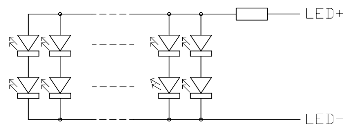
Backlight Circuit (No. of LEDs = 44pcs) Scale=free
