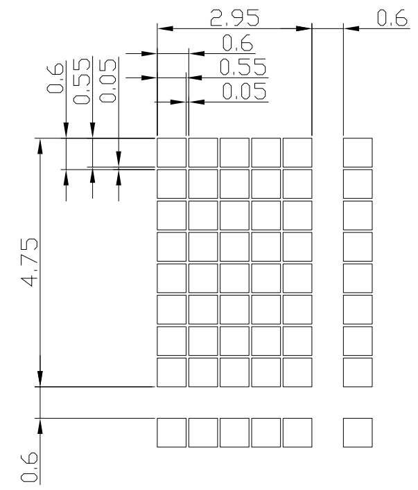
Pixels Details Scale=10/1
