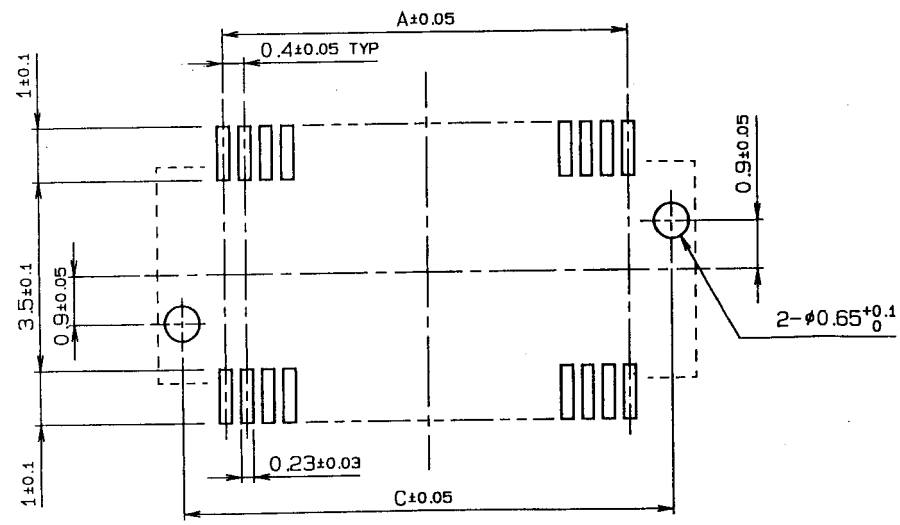
MOUNTING LAYOUT
