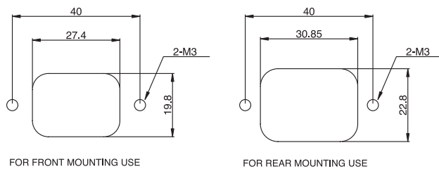
PANEL CUT-OUT
