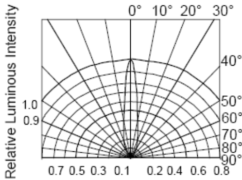
RADIATION DIAGRAM
