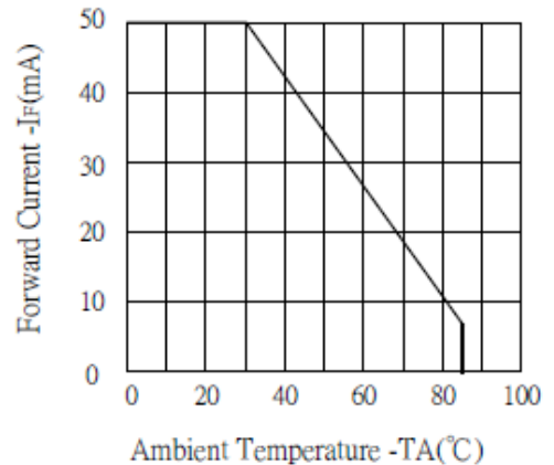
MAX FORWARD CURRENT Vs. AMBIENT TEMPERATURE
