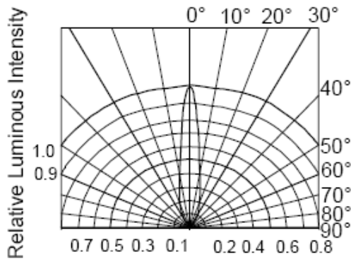
RADIATION DIAGRAM
